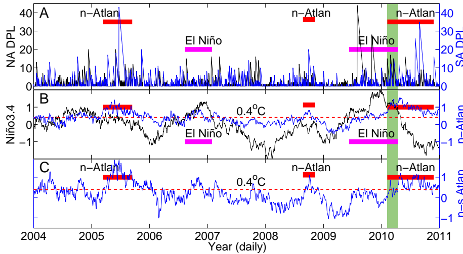
Fig. 3 Sensitivity of DPL to the SSTs of the Pacific and Atlantic. (A) DPL for the NA and SA. (B) SSTs of Niño3.4 and the tropical North Atlantic. The horizontal dashed line corresponds to a threshold of 0.4^{\circ}\text{C} , which is often used to define an El Niño event. Both a weak in 2006 and a strong El Niño events in 2010 are highlighted. Two time periods when the SST of the Atlantic Ocean is significantly above 0.4^{\circ}\text{C} are highlighted, together with a weak event in 2008. In 2010, a significantly overlapped window is highlighted between the El Niño event and the warming of SSTs in the North Atlantic. (C) Differential SST between the North and South Atlantic (a threshold of 0.4^{\circ}\text{C} is plotted for comparison).
