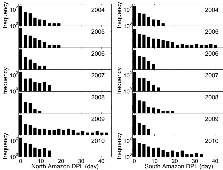
Fig. 2 Histograms of DPL in each year.
