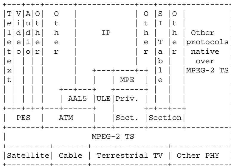
Figure 1: Overview of the MPEG-2 protocol stack
