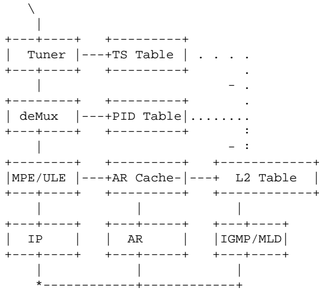
Figure 7: Receiver Processing Architecture
