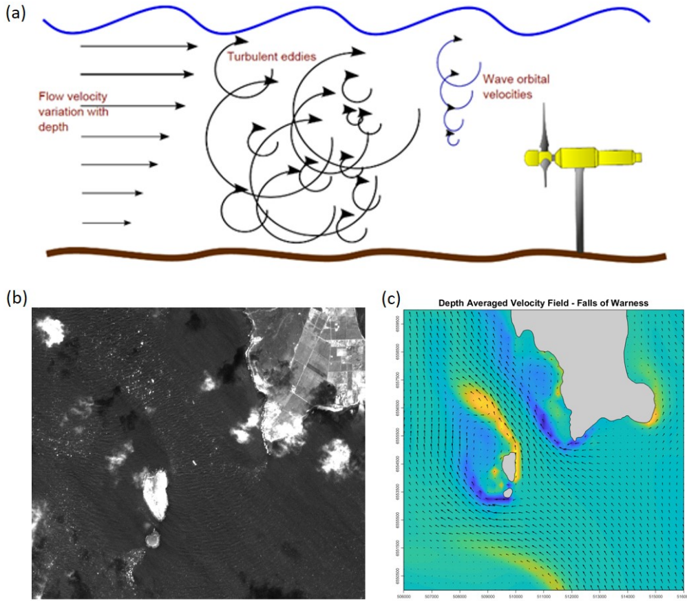
Figure 3: Site characterisation for tidal stream energy extractions needs to capture the full range of complex flow conditions. (a) The IEC/TS62600201.2015 in situ data specifications target the capture of the vertical variation in flow conditions, (b) but the spatial variations due to flow separation processes, as observed in satellite imagery (Sentinel2A channel B3 data, 21/04/2017), need to be considered, (c) this is where regional-scale modelling is required to extend the information content. The lower panels show the EMEC research site.
