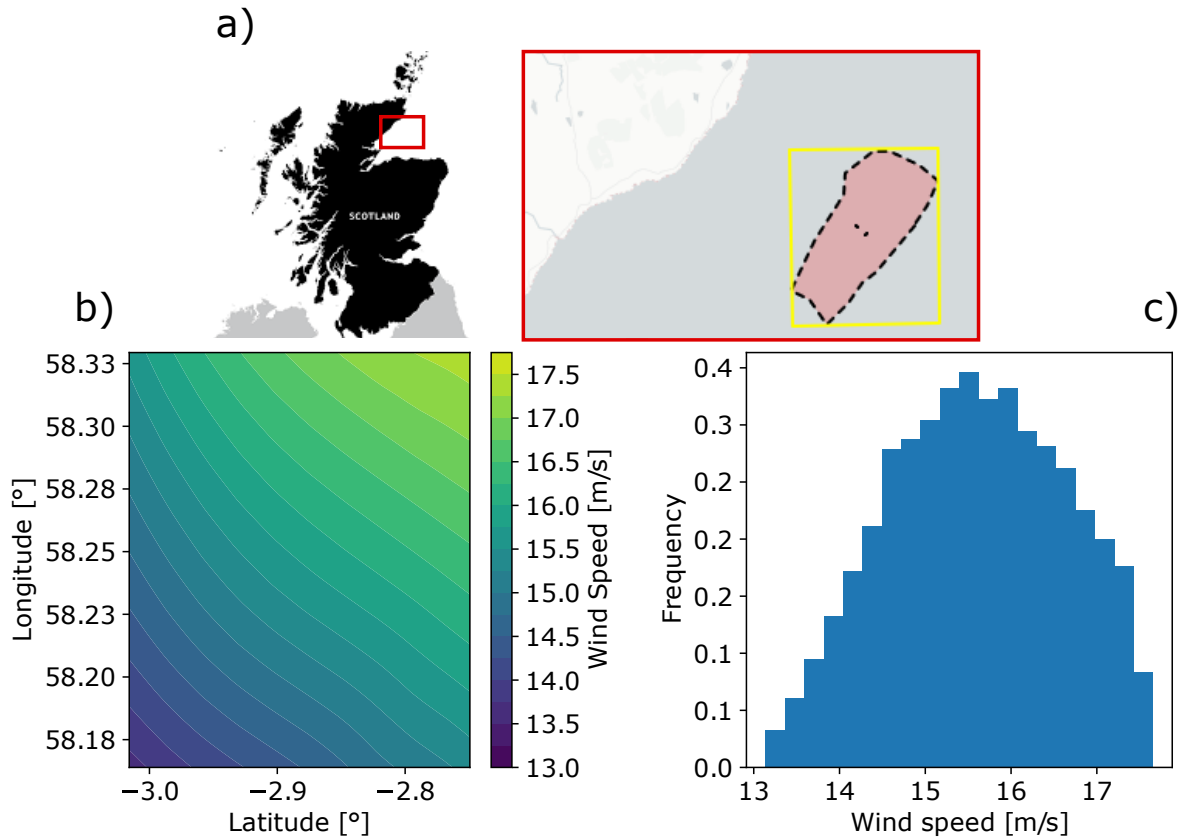
Figure 15: Example of spatial changes in wind speed within the area covered by an offshore wind farm. a) Wind farm location, off Scottish shores. b) Wind map for the area containing the wind farm presented in panel a). The wind field was extracted from maps for wind speed retrieved from SAR imagery available from DTU Wind Energy, DTU (2020). c) Normalized frequency distribution of the wind speed value observed in b), Zen et al. (2020).
