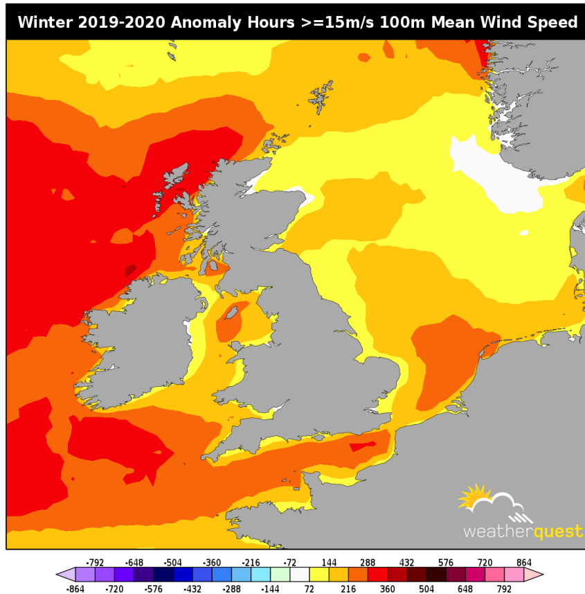
Figure 11: The number of hours with 100m mean wind speed \geq 15 m s -1 during Winter (December, January, February) 2019–2020 relative to the long-term ERA5 average. Source: Weatherquest Ltd.
