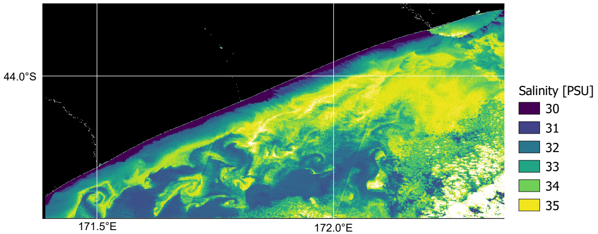
Figure 18: Sea surface salinity at Canterbury Bight (New Zealand), 100 m resolution. Results using Sentinel-2 Level1C imagery. Land is depicted in black, clouds in white. Extracted from Medina-Lopez (2020).
