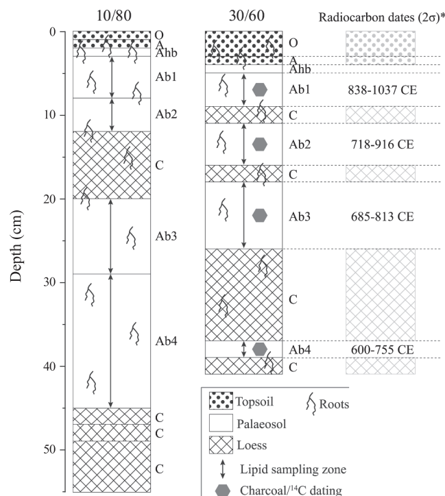
Fig. 2. Pedosequence description of soil test pits located at 10/80 and 30/60 (Fig. 1). Soil horizon notation corresponds to Jahn et al. (2006), A for buried palaeosol and C for wind-deposited sediment. Soil sampling for lipid analyses is described in detail in the Material and Method section. Radiocarbon dates are from Anderson et al. (2019).
