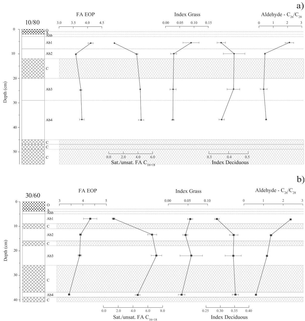
Fig. 5. Depth variations of fatty acid-based proxies and the C_{26}/C_{28} n -aldehyde ratio in palaeosols from sequences: (a) 10/80 and (b) 30/60. Proxy calculations are detailed in the Materials and method section.
