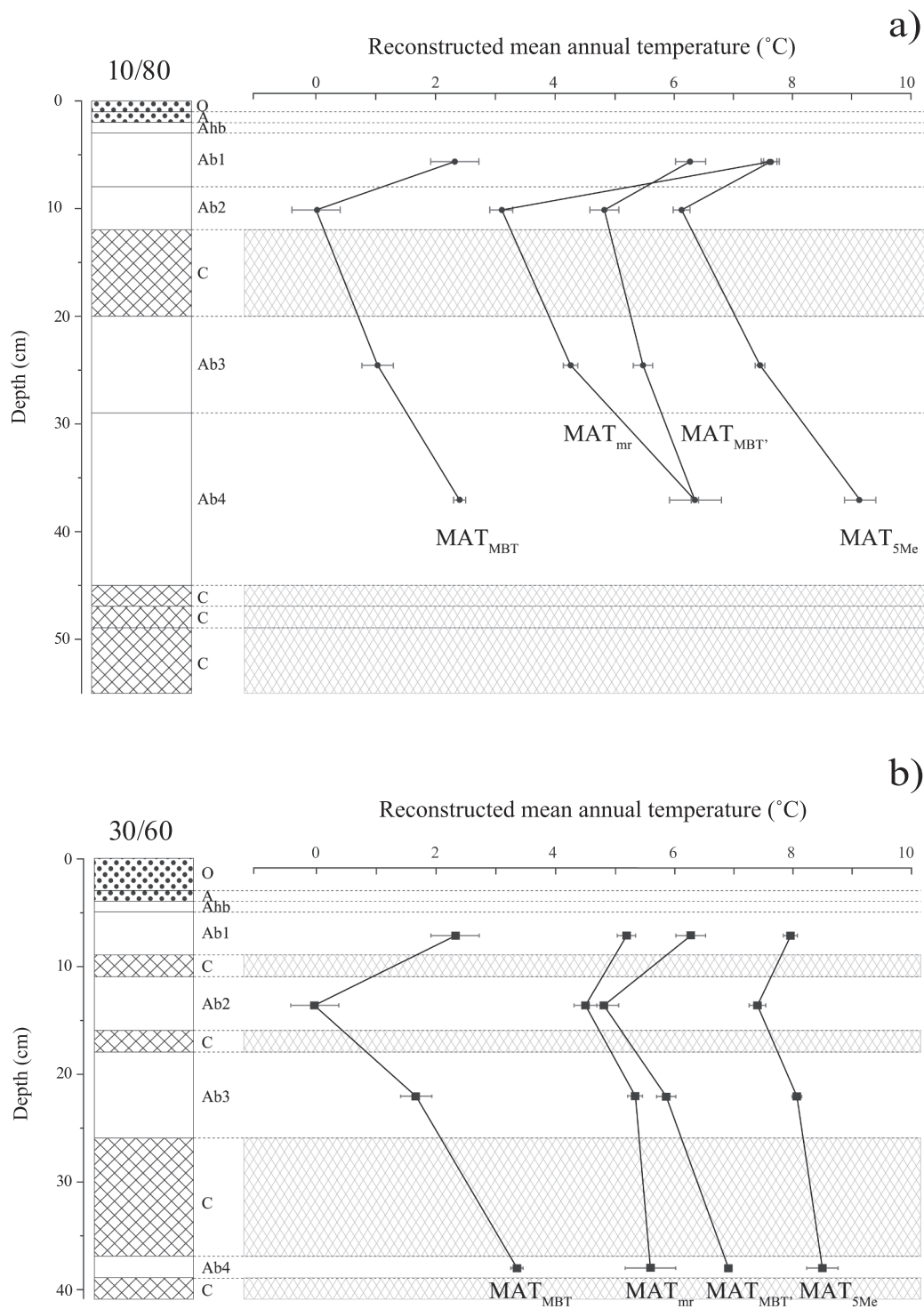
Fig. 7. Depth variations of reconstructed mean annual temperature (MAT) based on brGDGT-derived calibrations by Weijers et al. (2007; MAT MBT ), Peterse et al. (2012; MAT MBT' ) and De Jonge et al. (2014; MAT 5Me and MAT mr ) in palaeosols from sequences: (a) 10/80 and (b) 30/60. The different brGDGT calibrations are detailed in the Materials and methods section.
