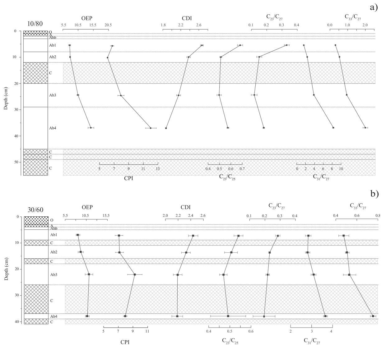
Fig. 4. Depth variations of n -alkane-based proxies in palaeosols from sequences: (a) 10/80 and (b) 30/60. Proxy calculations are detailed in the Materials and methods section.
