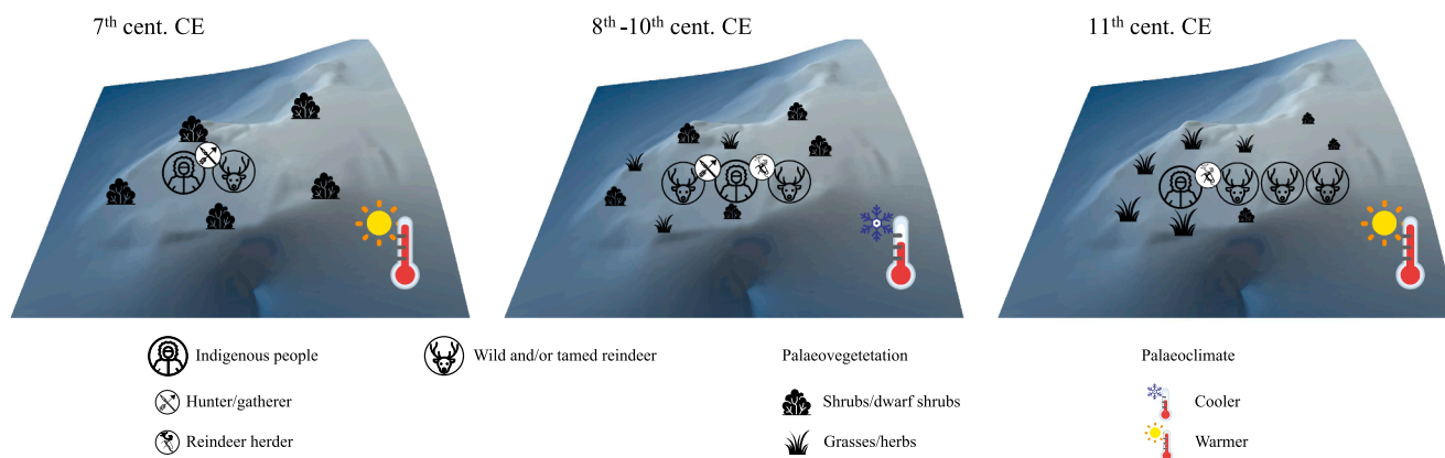
Fig. 8. Schematic representation of the evolution of human-animal-environment relationship and palaeoenvironmental conditions at IArte 6.
