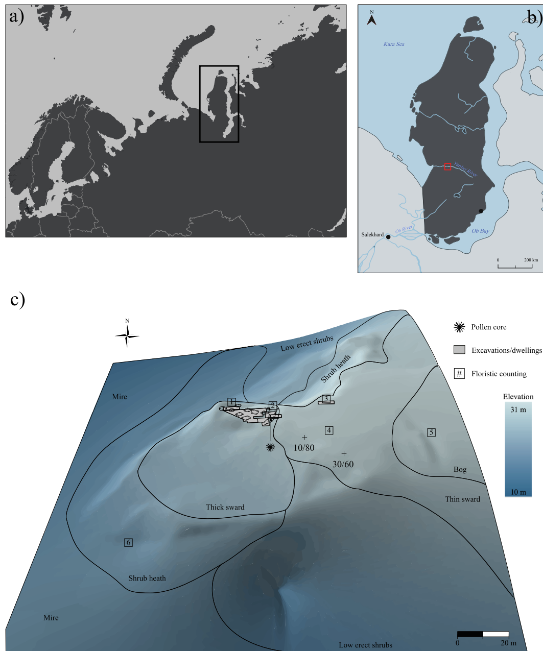
Fig. 1. Location of: (a) the Iamal Peninsula; (b) the IArte complex; (c) IArte 6 elevation model, including the locations of the loess-palaeosol sequences in test pits 10/80 and 30/60, the location of the different excavations conducted, modern vegetation community analysis (Bruce Forbes, personal data, quadrat numbers as in Supplementary Table S1) and the location of the soil monolith analysed for pollen (Anderson et al., 2019).
