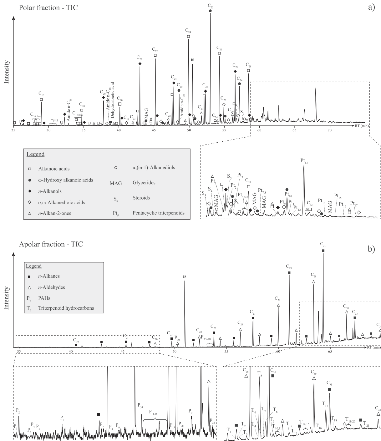
Fig. 3. Total ion current (TIC) chromatograms of the: (a) apolar and (b) polar fractions of a soil methodological replicate from the Ab4 horizon of sequence 30/60. C# shows the length of the n -alkyl chain. Compound names, formulae and other structural and spectral details can be found in Supplementary Table S3.
