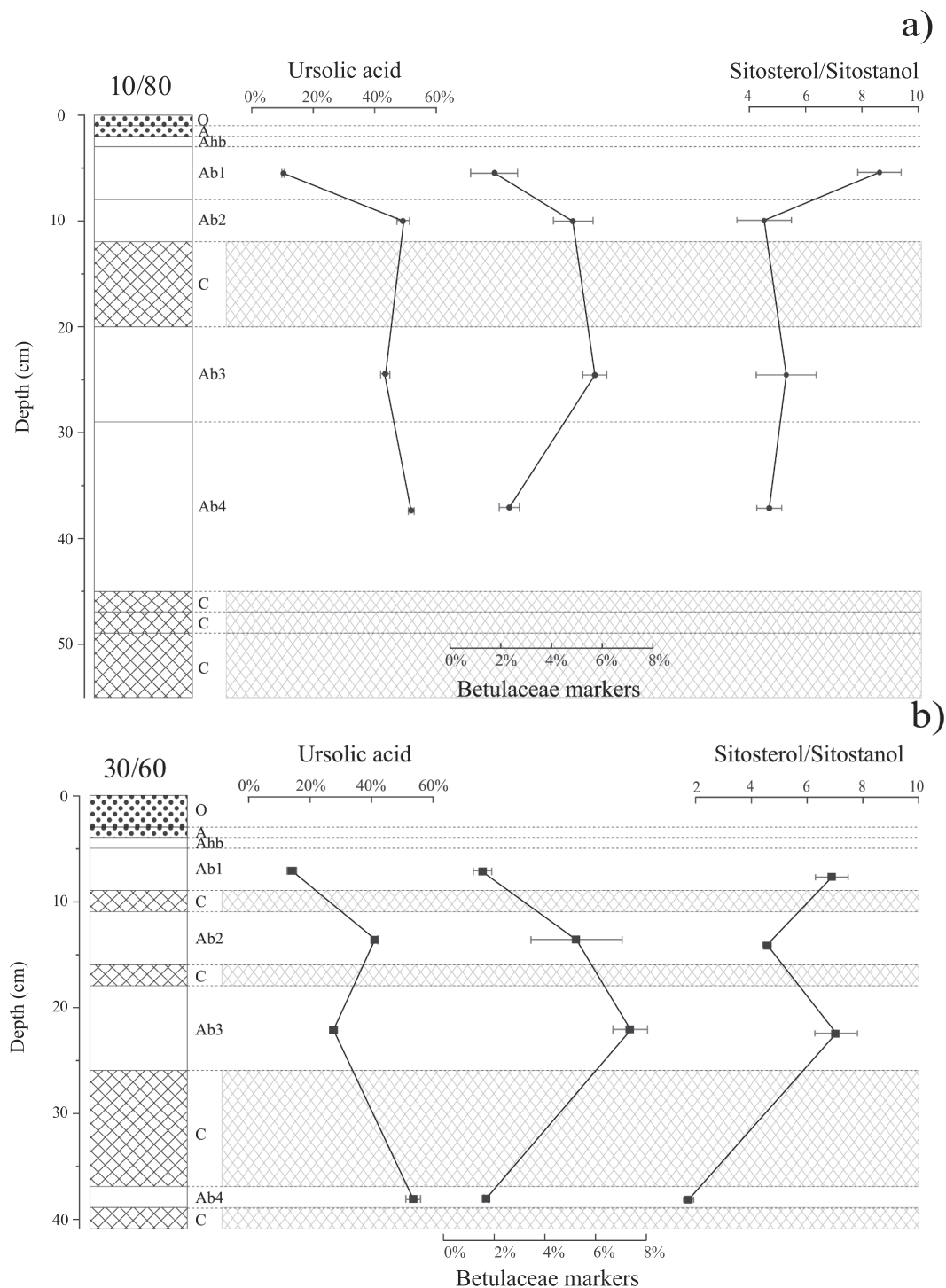
Fig. 6. Depth variations of ursolic acid, suggested Betulaceae biomarkers (sum of betulin, betulinic acid, lupeol and lupenone) and sitosterol/sitostanol ratio in palaeosols from sequences (a) 10/80 and (b) 30/60.
