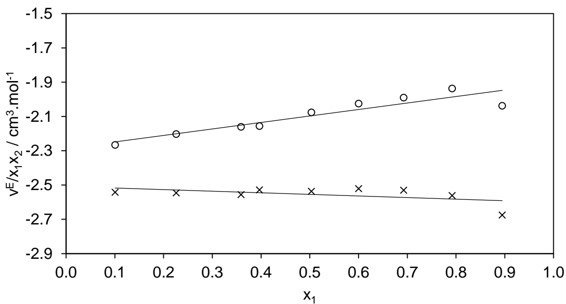
Figure 2: Plot of v^E/x_1x_2 for the furan(1) + MDEA(2) system as a function of the furan mole fraction x_1 at atmospheric pressure p and two different temperatures T : (unfilled circle) 278.15 K; (cross) 303.15 K; solid line, Redlich–Kister correlation.
