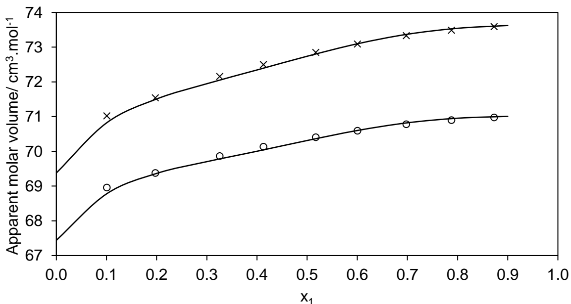
Figure 12: Calculated apparent molar volume using the Redlich–Kister correlation (solid line) and experimental apparent molar volume (symbols) of the furan(1) + DEG(2) system as a function of the furan mole fraction x_1 at atmospheric pressure p and two different temperatures T : (unfilled circle) 278.15 K, (cross) 303.15 K.
