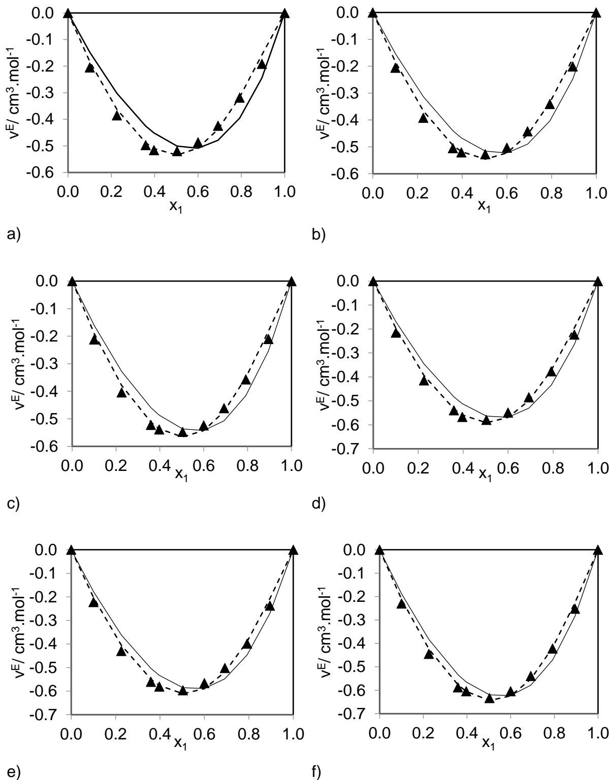
Figure 16: Excess volumes for the furan(1) + MDEA(2) binary system at T/ \text{K} = 278.15 (a), 283.15 (b), 288.15 (c), 293.15 (d), 298.15 (e), and 303.15 (f) as a function of the mole fraction x_1 . Symbols, experimental data; solid line, calculated using the PFP model with constant value of X_{12} ; dashed line, calculated with the PFP model with X_{12} being composition dependent.
