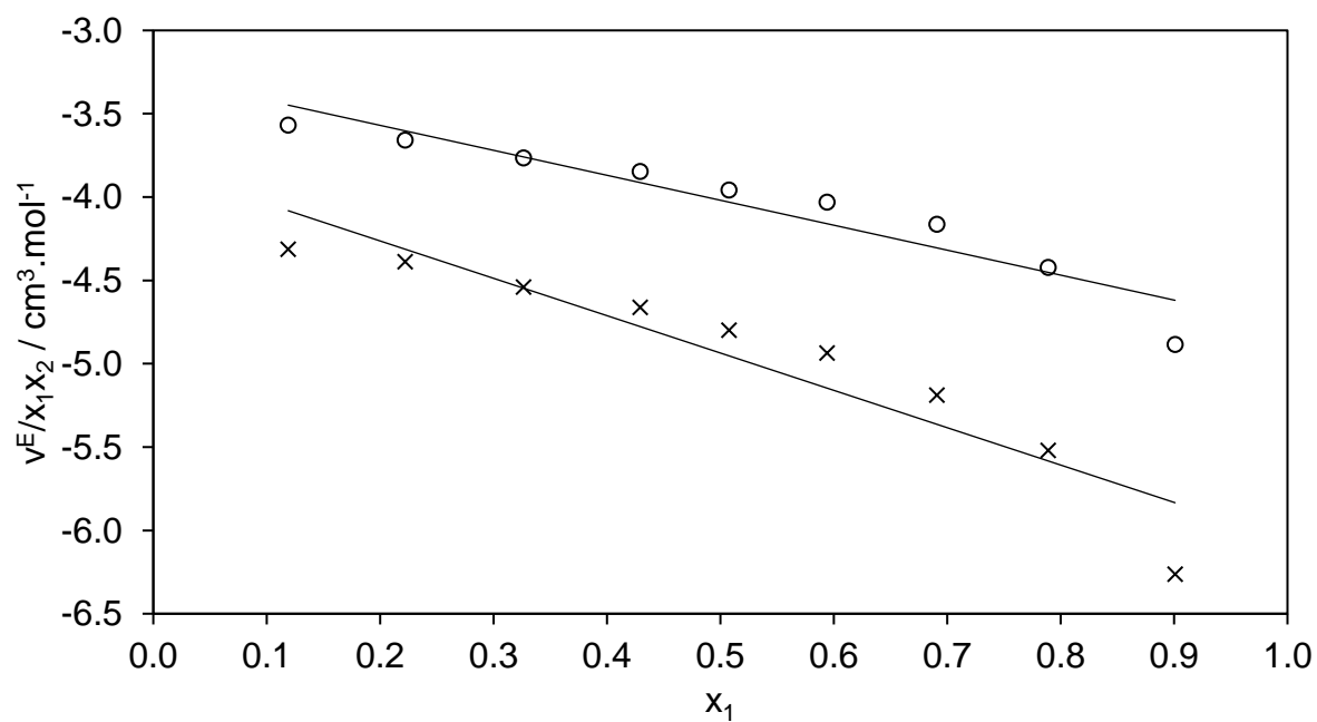
Figure 6: Plot of v^E/x_1 x_2 for the furan(1) + TEG(2) system as a function of the furan mole fraction x_1 at atmospheric pressure p and two different temperatures T : (unfilled circle) 278.15 K; (cross) 303.15 K; solid line, Redlich–Kister correlation.
