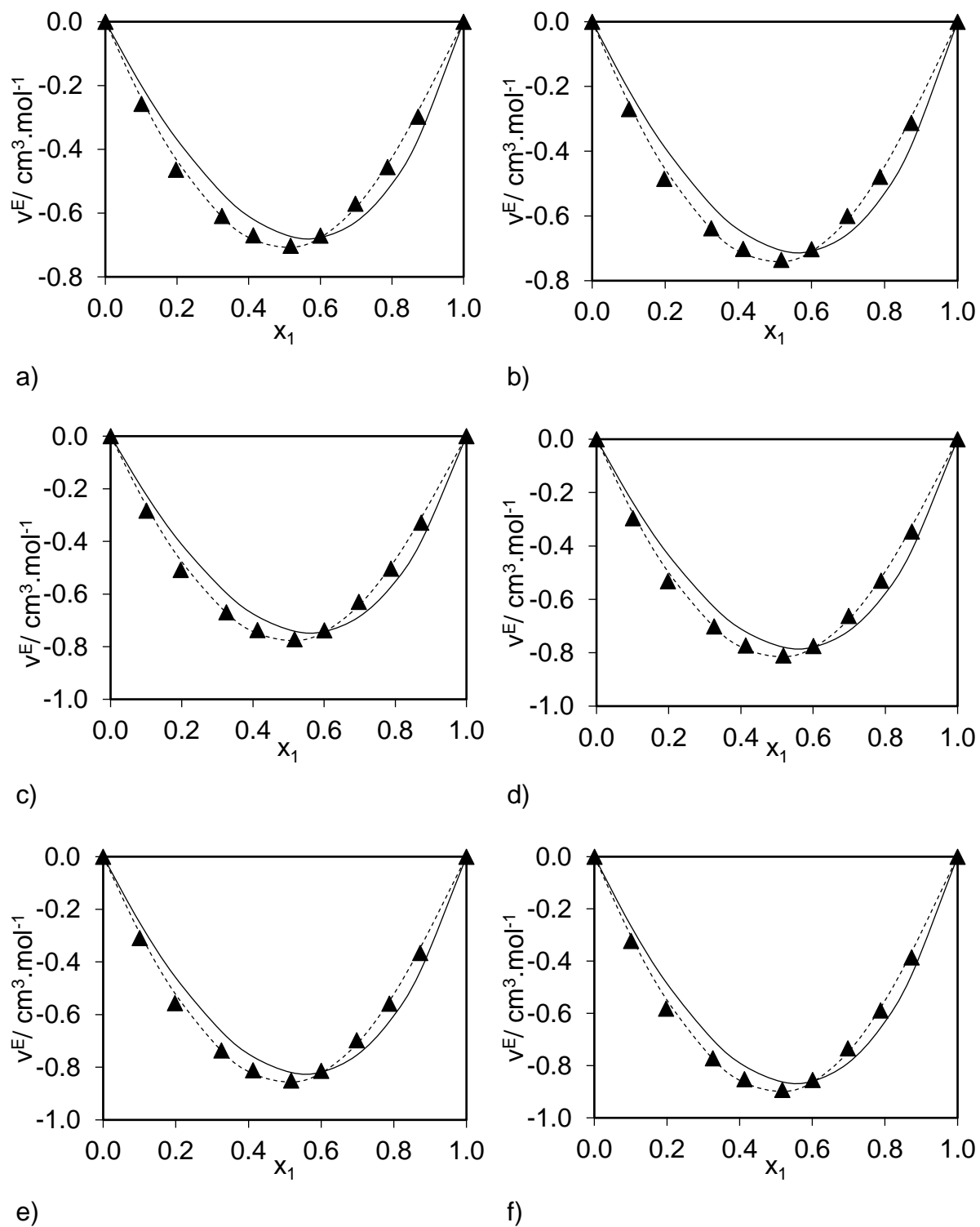
Figure 17: Excess volumes for the furan(1) + DEG(2) binary system at T/ \text{K} = 278.15 (a), 283.15 (b), 288.15 (c), 293.15 (d), 298.15 (e), and 303.15 (f) as a function of the mole fraction x_1 . Symbols, experimental data; solid line, calculated using the PFP model with constant value of X_{12} ; dashed line, calculated with the PFP model with X_{12} being composition dependent.
