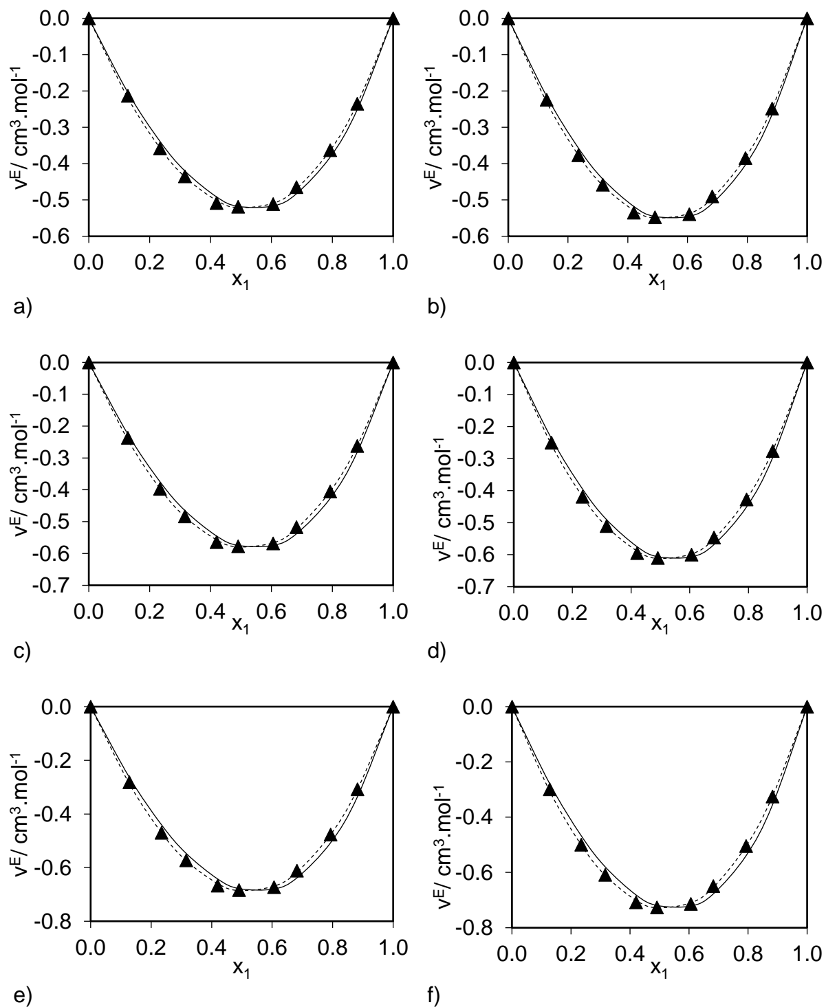
Figure 20: Excess volumes for the DMF(1) + DMA(2) binary system at T/ \text{K} = 283.15 (a), 293.15 (b), 303.15 (c), 323.15 (d), 333.15 (e), and 343.15 (f) as a function of the mole fraction x_1 . Symbols, experimental data; solid line, calculated using the PFP model with constant value of X_{12} ; dashed line, calculated with the PFP model with X_{12} being composition dependent.
