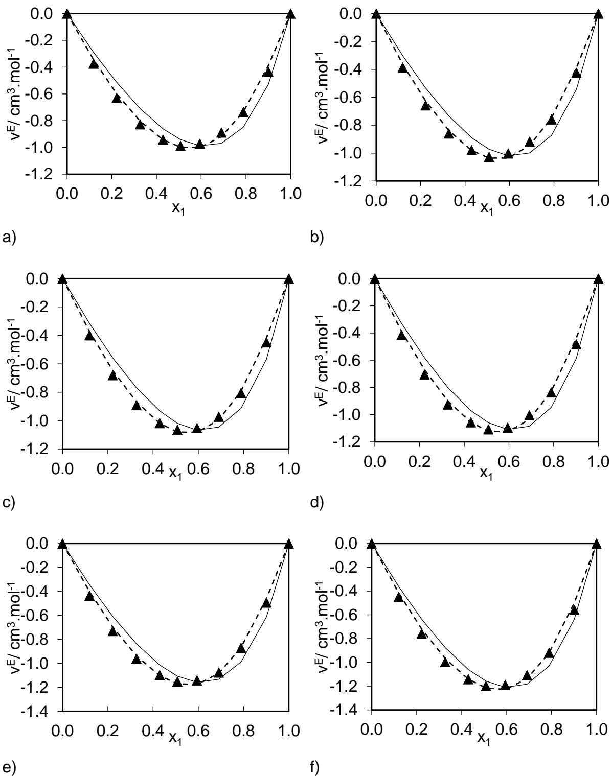
Figure 18: Excess volumes for the furan(1) + TEG(2) binary system at T/ K=278.15 (a), 283.15 (b), 288.15 (c), 293.15 (d), 298.15 (e), and 303.15 (f) as a function of the mole fraction x_1 . Symbols, experimental data; solid line, calculated using the PFP model with constant value of X_{12} ; dashed line, calculated with the PFP model with X_{12} being composition dependent.
