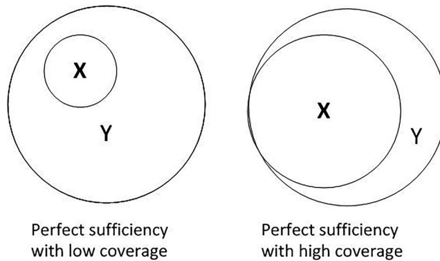
Figure 2. Venn diagrams showing low and high coverage.
