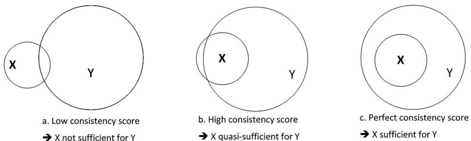
Figure 1. Venn diagrams representing various degrees of sufficiency of X for Y.
