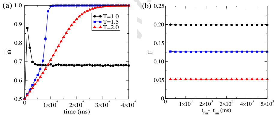
Figure 5: (Colour online)(a) \bar{\omega} as a function of the time and (b) F versus t_{\text{fin}} - t_{\text{ini}} for T = 1 (black circles), T = 1.5 (blue squares), and T = 2 (red triangles). We consider t_{\text{ini}} = 4 \times 10^5 and \sigma = 0.9 .
