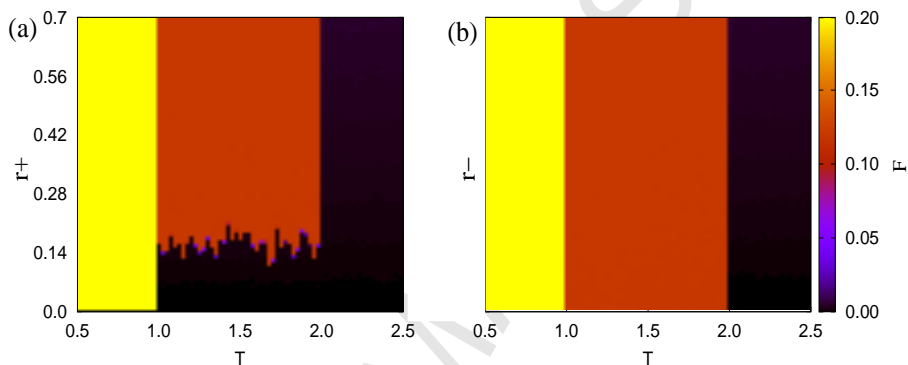
Figure 6: (Colour online) Figs (a) and (b) show r_+ and r_- as a function of T , respectively, where \sigma = 0.9 and the colour bar represents F .
