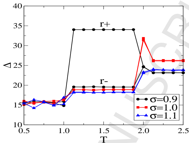
Figure 7: (Colour online) \Delta \times T for the network with plasticity and T \in [0.5, 2.5] , where \sigma = 0.9 (black circles), \sigma = 1.0 (red squares), and \sigma = 1.1 (blue triangles).
