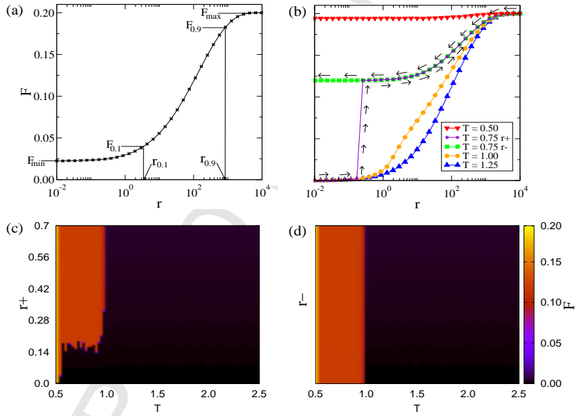
Figure 2: (Colour online) The average firing rate F for different configurations in the values of T and r in a neural network with N = 10^4 . In Fig. (a), we have \sigma = 1.1 and T = 1.5 and we show F as a function of r , where the input rates r_{0.1} and r_{0.9} are obtained for 10% and 90% of the interval between F_{\min} and F_{\max} , respectively. Figure (b) exhibits results for different values of threshold T , while \sigma is maintained constant equal to 0.9. For T = 0.75 , T values will depend on how the parameter r is varied during the emulations. Increased increments produce the values indicated by the branch r^+ , decreasing values by the branch r^- . Figures (c) and (d) show the values of F , represented by the colour code of the side bar, for \sigma = 0.9 when r values are gradually incremented (c), or gradually decremented (d).
