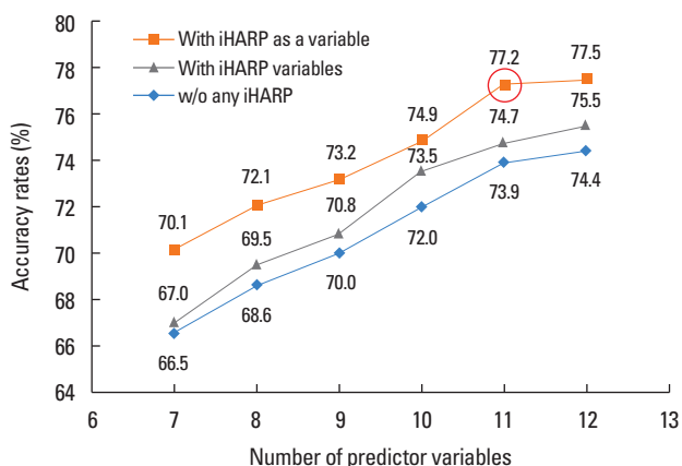
Fig. 5. Predictive accuracy rates corresponding to the number of predictor variables for iHARP variable combinations.
