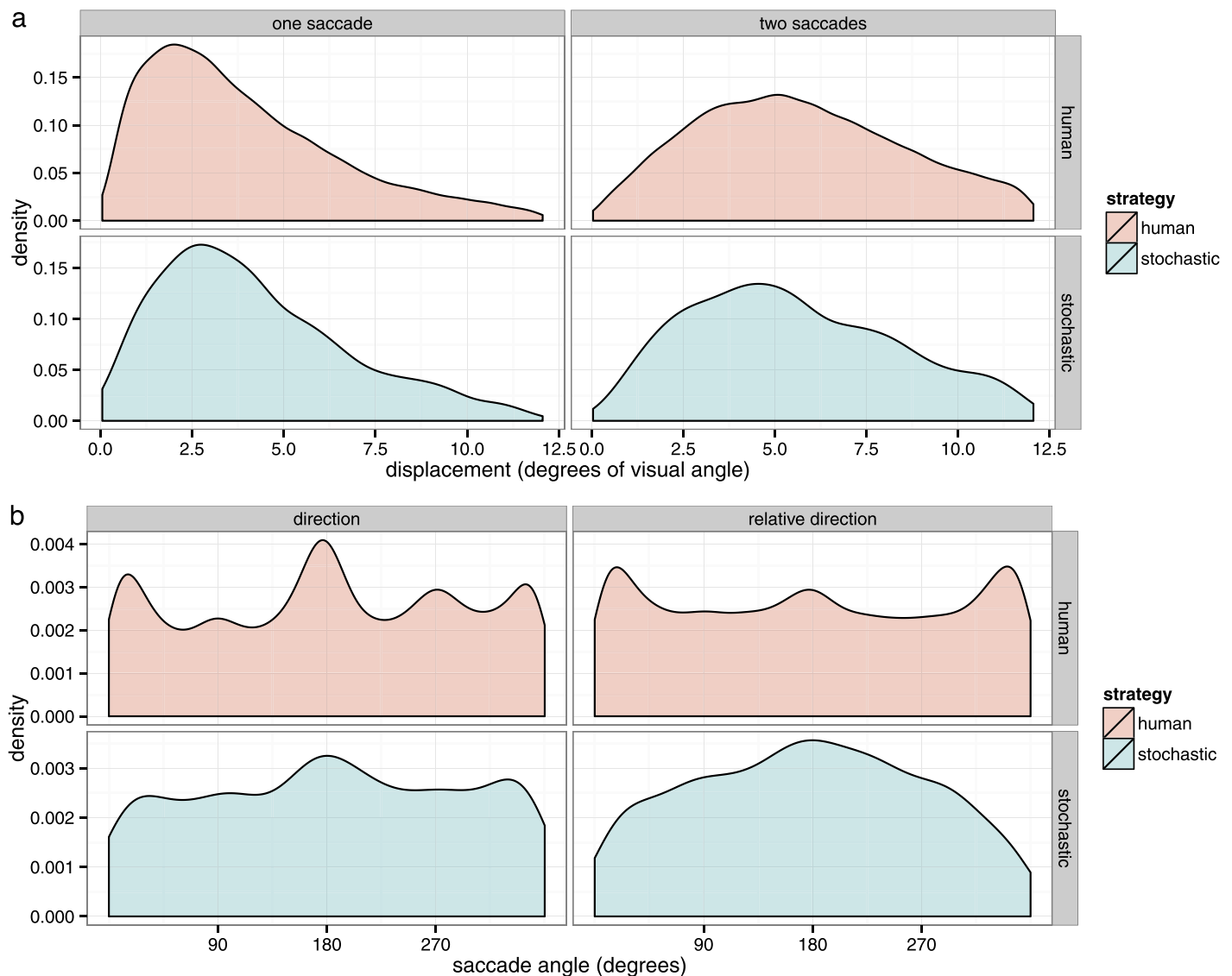
Figure 9. (a) Displacement over one and two saccades. (b) Absolute and relative direction of saccades. The fact that the stochastic model matches the distribution of displacement and direction over a single saccade is a direct result of sampling from empirical data and is therefore unsurprising.
