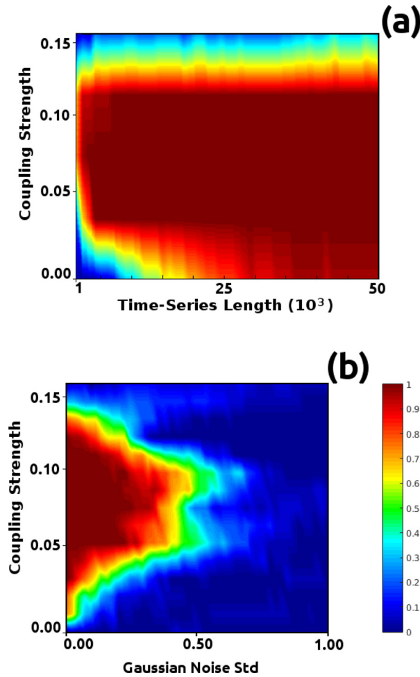
FIG. 3. Network inference based on logistic maps, for different coupling and noise strengths. Panel (a) shows the parameter space of the percentage of reconstruction (0%—blue and 100%—dark red) for different coupling strengths versus data lengths. Panel (b) is similar to panel (a) for different coupling strengths versus the standard deviation of the normal distribution of the noise added.
