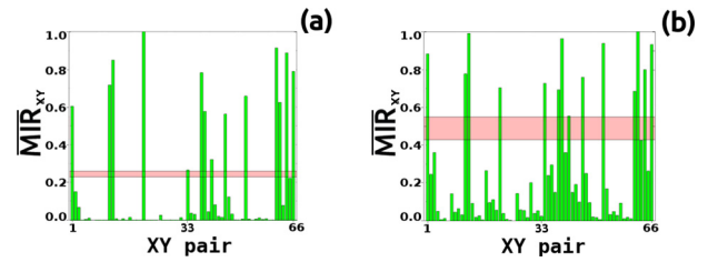
FIG. 4. Network inference for a network of nodes with a HR neural dynamics for different electrical couplings. Panels (a) and (b) show the bar plots of the percentage of inference for g_l = 0.05 and g_l = 0.1 , respectively. The red bands show the range of thresholds for which the original network is inferred with a 100% success.
