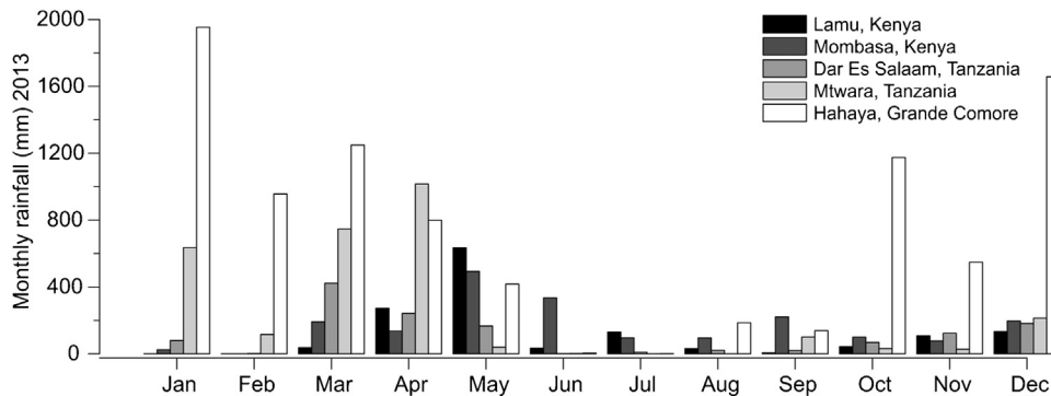
Fig. 6. Comparative monthly rainfall totals for 2013 indicating the annual variation in rainfall across seasons from Lamu in northern Kenya to Mtwara in southern Tanzania and Hahaya on Grande Comore island.
