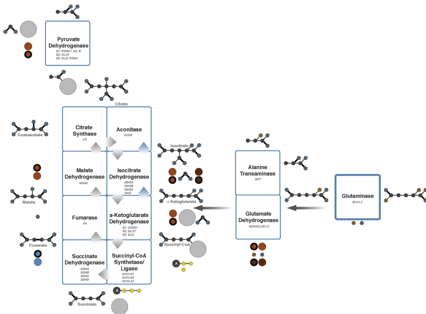
Fig. 2. Schematic of the TCA cycle and glutaminolysis. Enzymes altered in cancer are shown in bold. Reductive direction of the TCA cycle shown with blue arrows. Color scheme: carbon, gray; oxygen, blue; phosphate, yellow; nitrogen, brown; adenosine, A; coenzyme A, light gray; NAD + /NADH, orange; NADP + /NADPH, brown; FAD/FADH 2 , blue; single bonds, thin; double bonds, bold.
