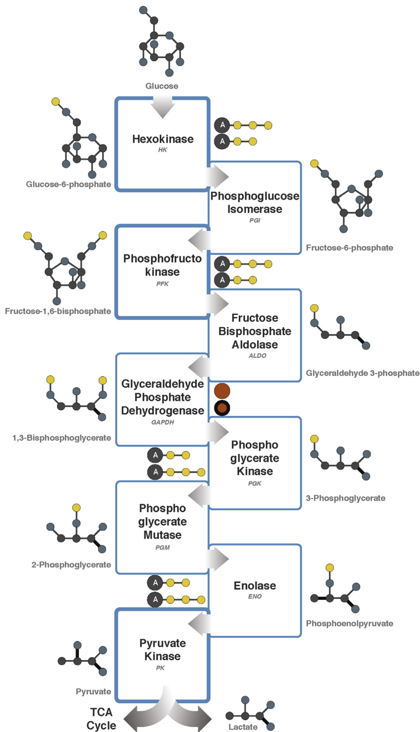
Fig. 1. Schematic of glycolysis. Enzymes altered in cancer are shown in bold. Color scheme: carbon, gray; oxygen, blue; phosphate, yellow; adenosine, A; NAD + /NADH, orange; single bonds, thin; double bonds, bold.
