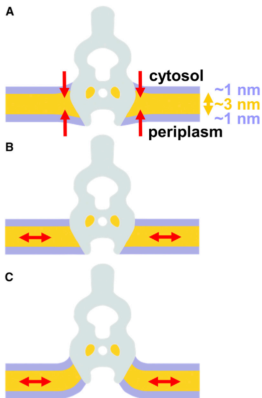
Figure 8. Interaction of Ynal with the Membrane
