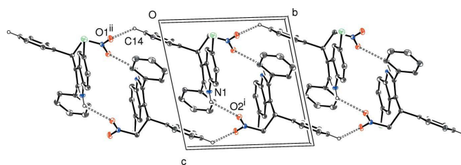
Figure 8 Fragment of an [010] chain in the crystal of (IV) linked by N-H\cdots O and C-H\cdots O hydrogen bonds (double-dashed lines). Symmetry codes as in Table 4.
