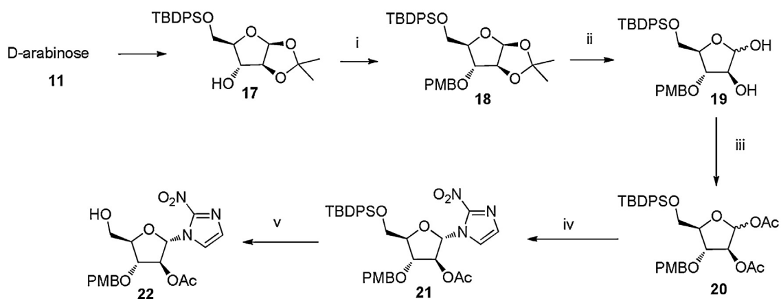
Scheme 8. Reagent and conditions: (i) PMBCl, NaH, TBAI, DMF, 0° to rt (72%); (ii) aqueous TFA 50%, DCM (52%), rt; (iii) Ac 2 O, Py, rt (100%); (iv) 1-TES-2-nitroimidazole (4), TfOTES, MeCN, -20 °C to -8 °C (76%); and (v) KF, PhCOOH, MeCN, 75 °C (95%).
